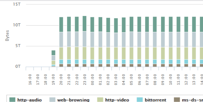
Top 5 Bandwidth Consuming Apps (last 24 hours)
